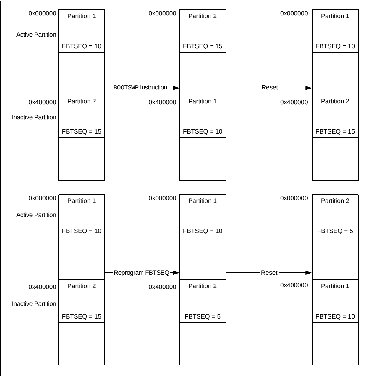
FIGURE 6-1: RELATIONSHIP BETWEEN PARTITIONS 1 AND 2 AND ACTIVE/INACTIVE PARTITIONS
