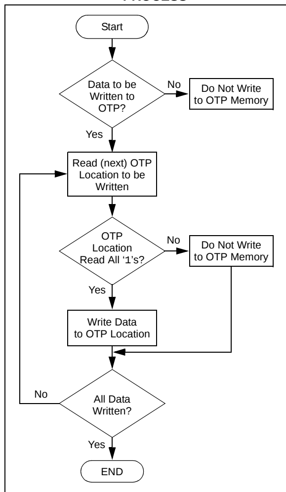
FIGURE 3-9: OTP PROGRAMMING PROCESS
