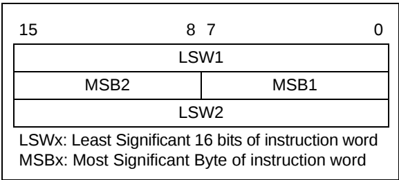
FIGURE 5-4: PACKED INSTRUCTION WORD FORMAT
