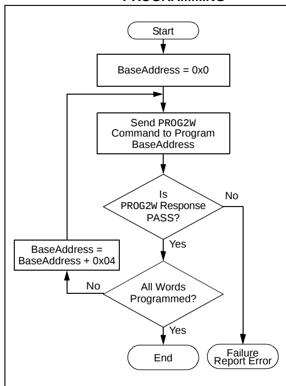
FIGURE 4-4: FLOWCHART FOR DOUBLE-WORD PROGRAMMING
